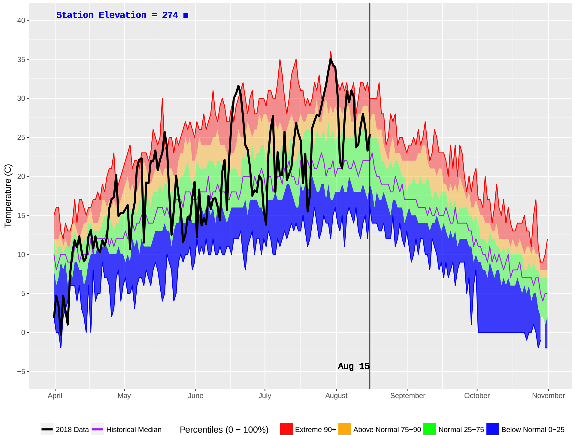
CEDARVALE (429) : Historical (1982–2016) and Current (2018) Daily Temperature
